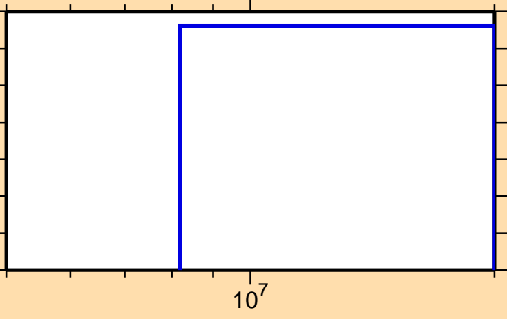
\sigma vs. E for ^{86}\text{Nb}(n,2n)
