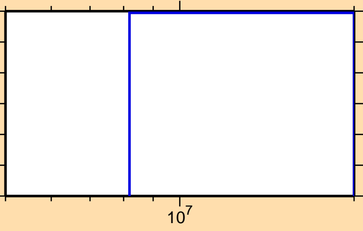
\sigma vs. E for ^{86}\text{Nb}(n,\text{pt})
