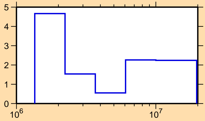
\Delta\sigma/\sigma vs. E for ^{87}\text{Nb}(n,n\text{nonel.})
