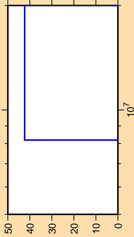
\Delta\sigma/\sigma vs. E for ^{87}\text{Nb}(n,nd)
