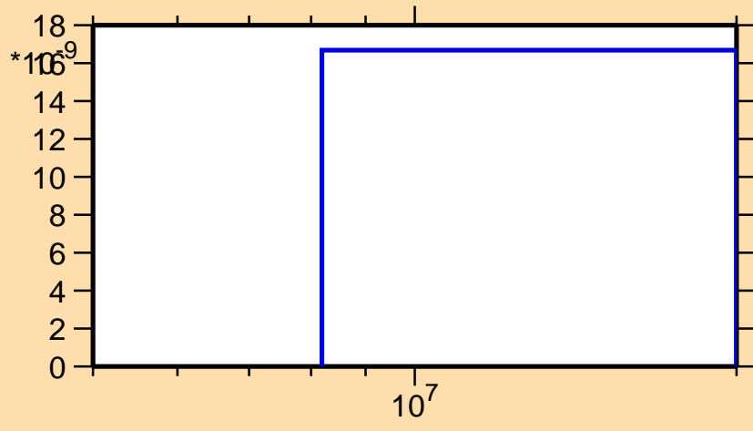
\sigma vs. E for ^{87}\text{Nb}(n,nd)
