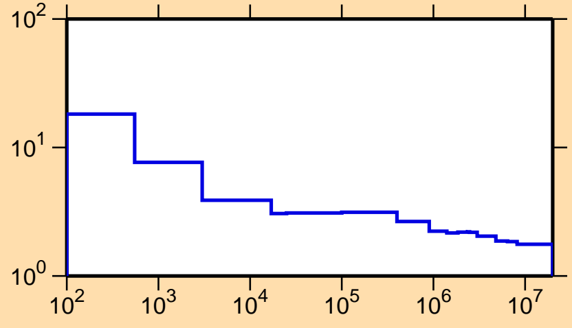
\sigma vs. E for ^{87}\text{Nb}(n,\text{nonel.})
