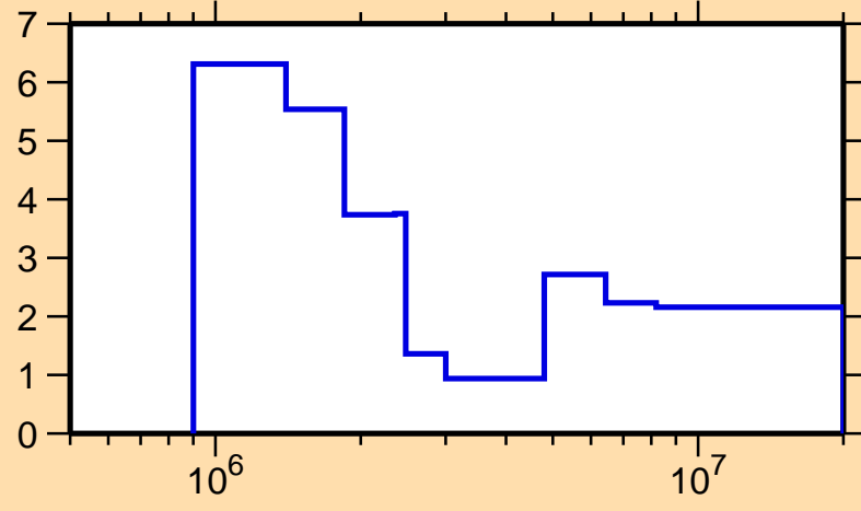
\Delta\sigma/\sigma vs. E for ^{87}\text{Nb}(n,n\text{onel.})
