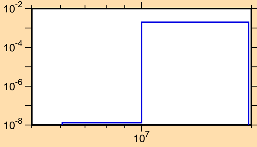
\sigma vs. E for ^{87}\text{Nb}(n,n\alpha)
