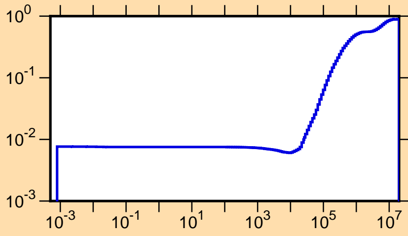
\mu vs. E for ^{88}\text{Nb}(\text{mt251})
