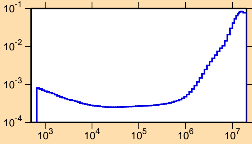
\sigma vs. E for ^{88}\text{Nb}(n,\alpha)
