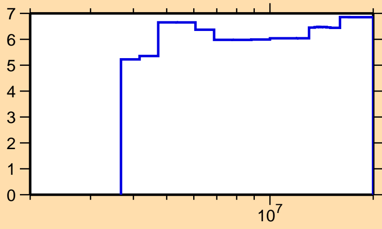
\Delta\sigma/\sigma vs. E for ^{88}\text{Nb}(n,n\text{onel.})
