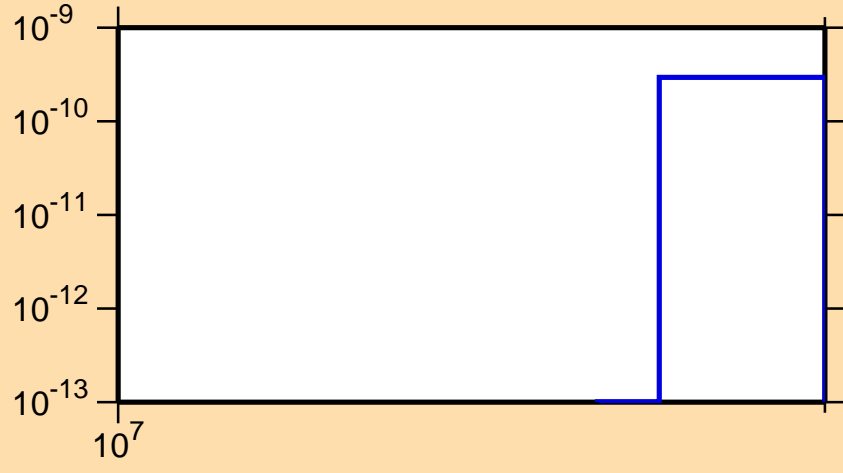
\sigma vs. E for ^{88}\text{Nb} (mt 34)
