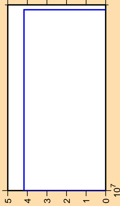
\Delta\sigma/\sigma vs. E for ^{88}\text{Nb} (mt 34)
