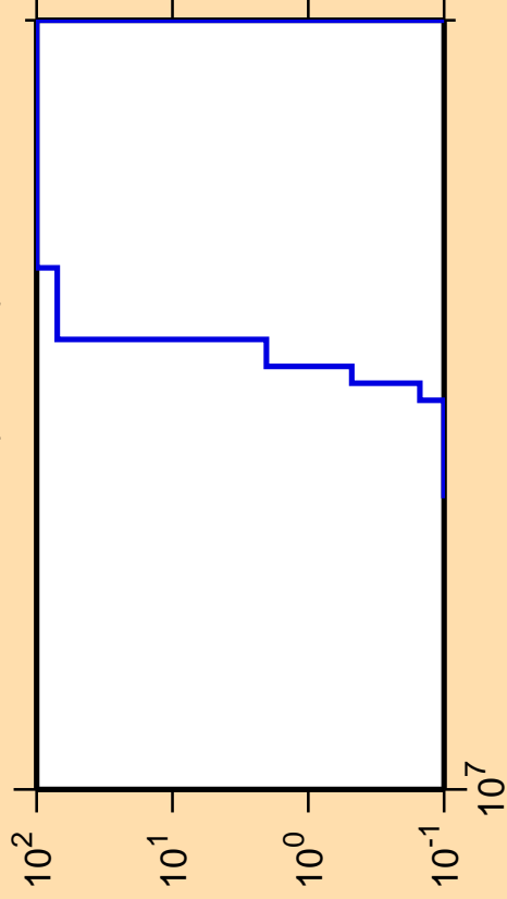
\Delta\sigma/\sigma vs. E for ^{89}\text{Nb} (mt117)
