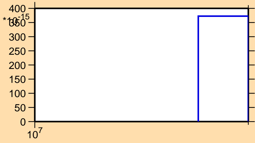
\sigma vs. E for ^{89}\text{Nb}(n,nt)
