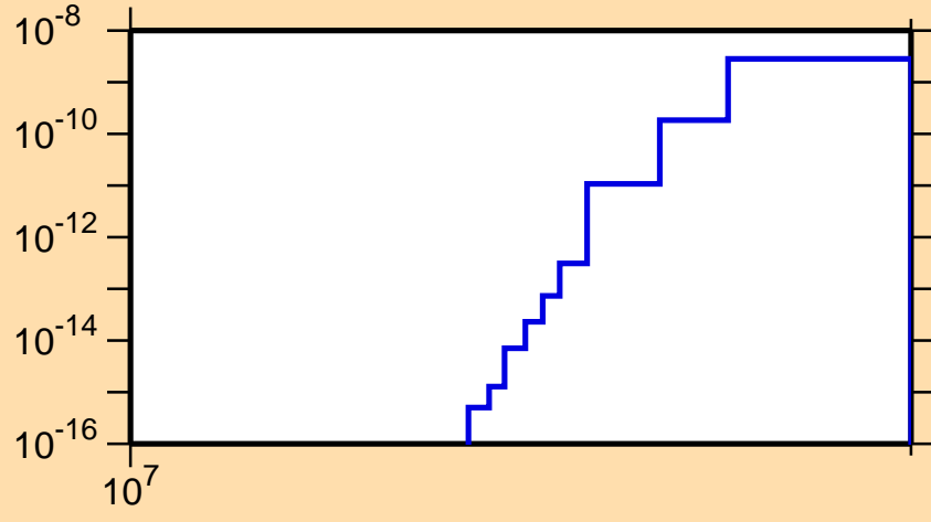
\sigma vs. E for ^{89}\text{Nb} (mt117)
