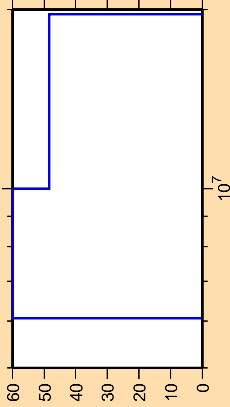
\Delta\sigma/\sigma vs. E for ^{89}\text{Nb}(n,n\alpha)
