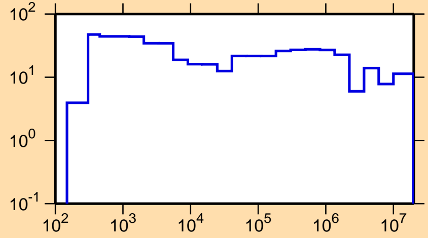
\Delta\sigma/\sigma vs. E for ^{89}\text{Nb}(n,\text{el.})
