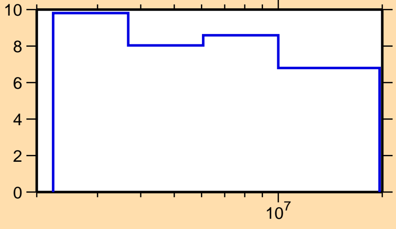
\Delta\sigma/\sigma vs. E for ^{89}\text{Nb}(n,n\text{nonel.})
