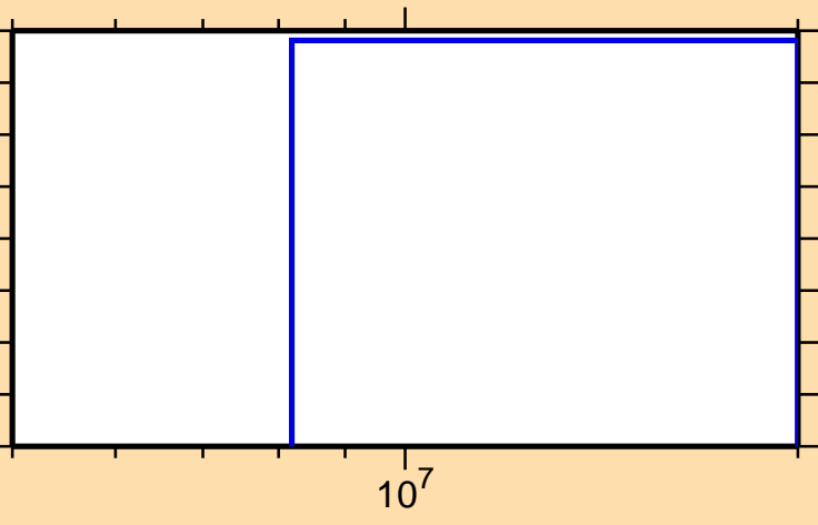
\sigma vs. E for ^{89}\text{Nb}(n,2n)
