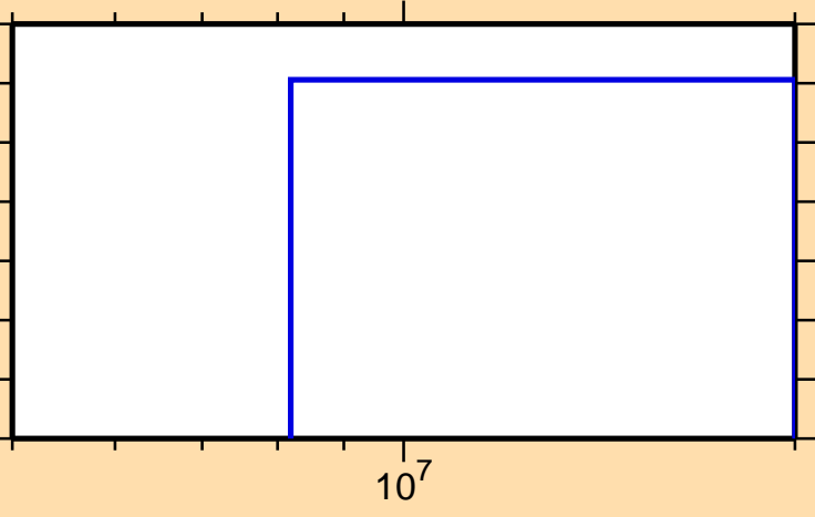
\sigma vs. E for ^{89}\text{Nb}(n,nt)
