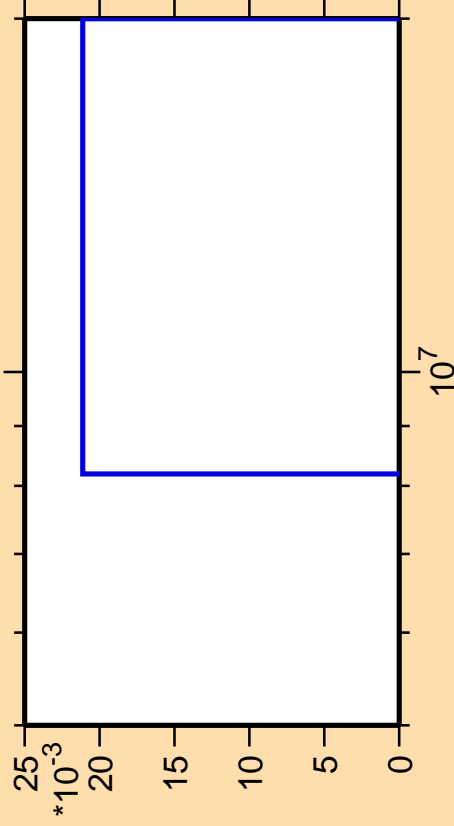
\Delta\sigma/\sigma vs. E for ^{89}\text{Nb}(n,nt)
