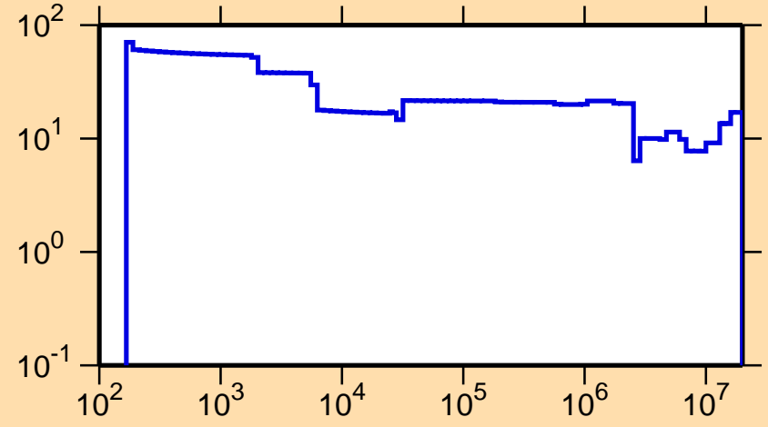
\Delta\sigma/\sigma vs. E for ^{90}\text{Nb}(n,\text{el.})
