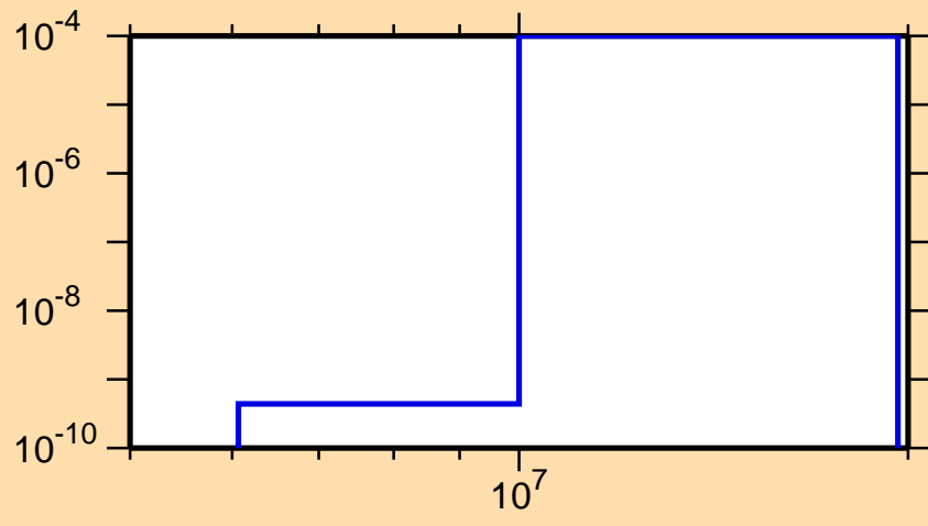
\sigma vs. E for ^{90}\text{Nb}(n,t)
