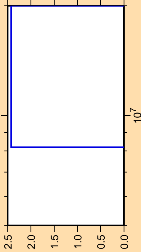
\Delta\sigma/\sigma vs. E for ^{90}\text{Nb}(n,\text{pt})
