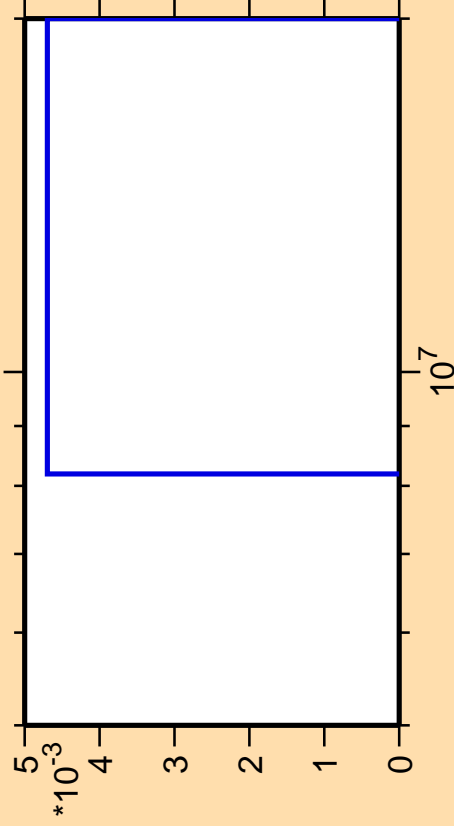
\Delta\sigma/\sigma vs. E for ^{90}\text{Nb} (mt 34)
