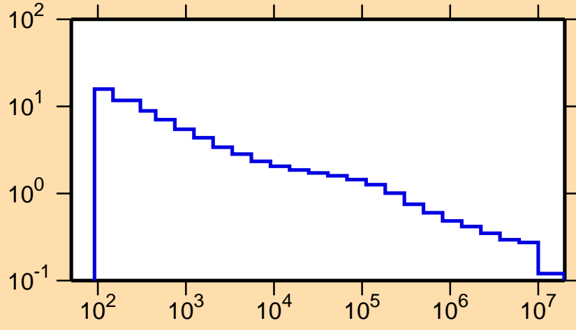
\sigma vs. E for ^{90}\text{Nb}(n,p)
