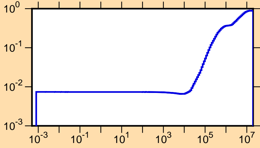
\mu vs. E for ^{91}\text{Nb}(\text{mt251})
