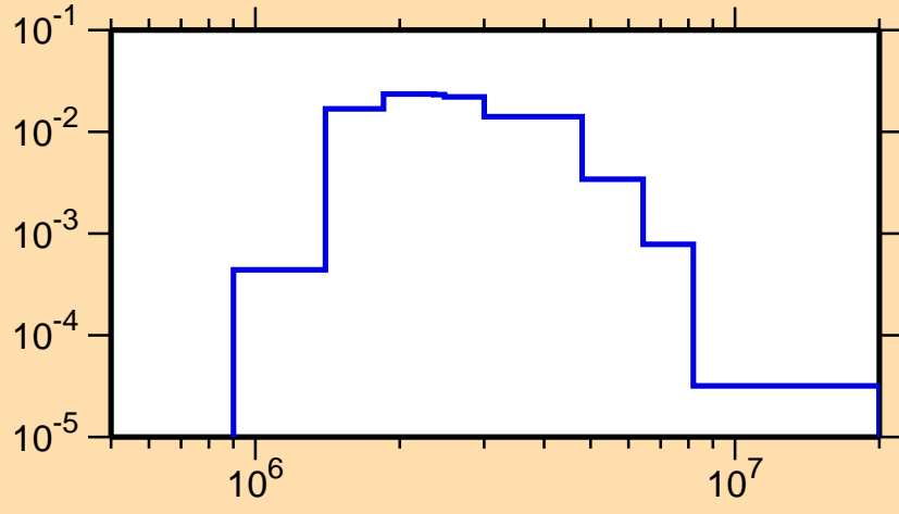
\sigma vs. E for ^{91}\text{Nb}(n,n_4)
