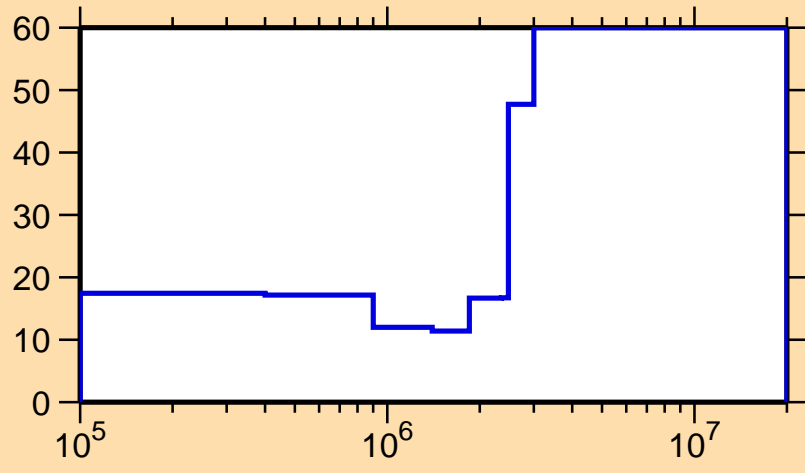
\Delta\sigma/\sigma vs. E for ^{91}\text{Nb}(n,n_1)
