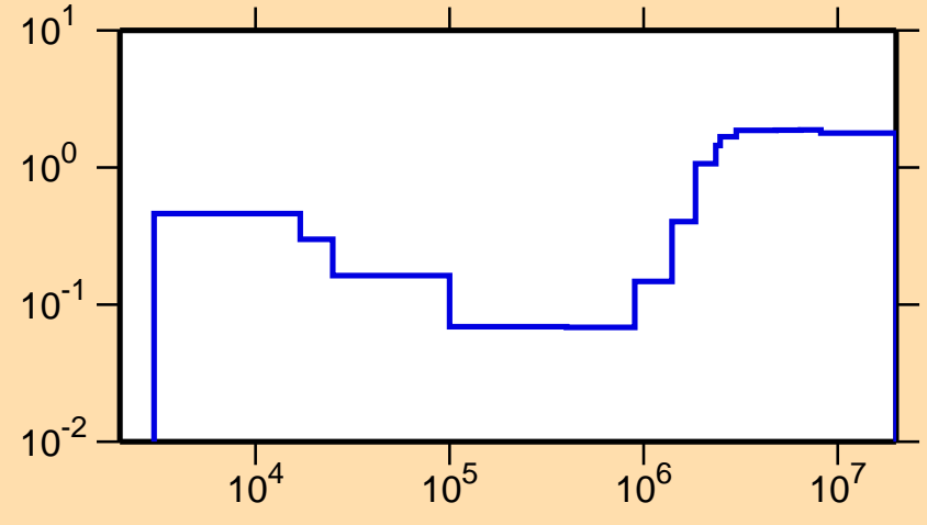
\sigma vs. E for ^{91}\text{Nb}(n,\text{nonel.})
