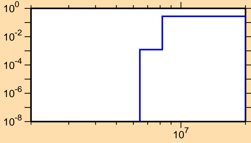
\sigma vs. E for ^{91}\text{Nb}(n,np)
