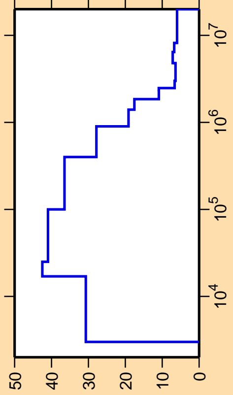
\Delta\sigma/\sigma vs. E for ^{91}\text{Nb}(n,\text{nonel.})
