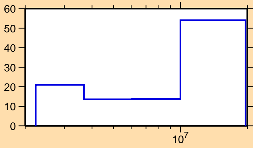
\Delta\sigma/\sigma vs. E for ^{91}\text{Nb}(n,n\text{cont.})
