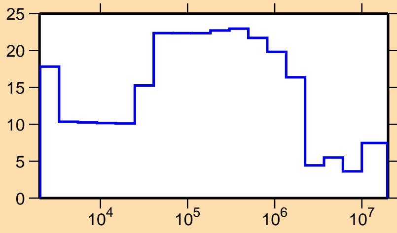
\Delta\sigma/\sigma vs. E for ^{91}\text{Nb}(n,\text{tot.})
