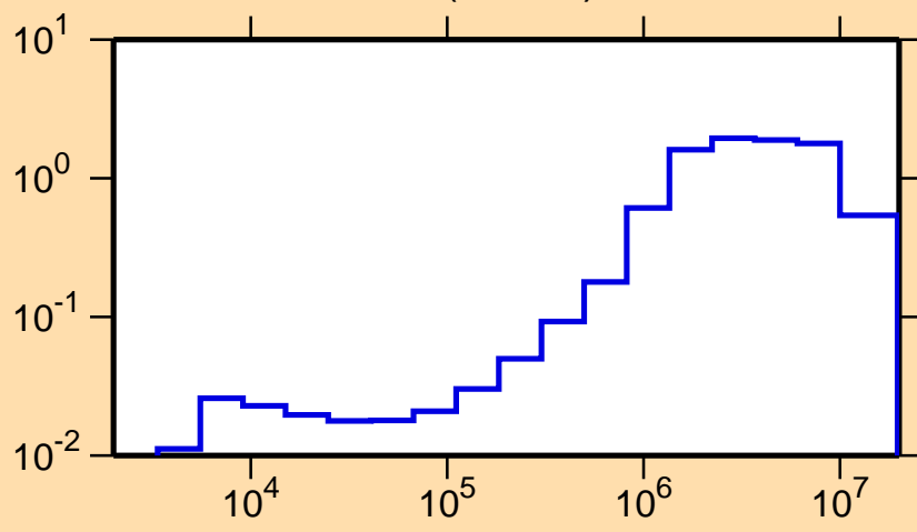
\sigma vs. E for ^{91}\text{Nb}(n,\text{inel.})
