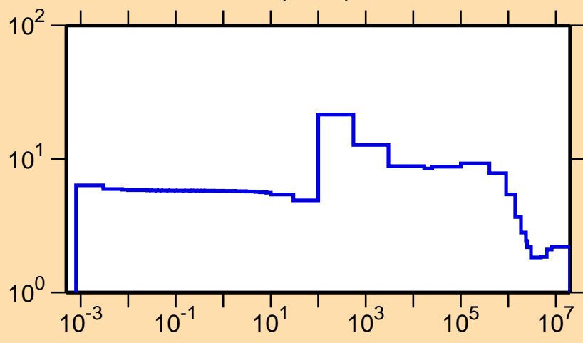
\sigma vs. E for ^{91}\text{Nb}(n,\text{el.})
