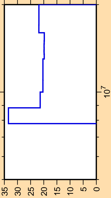
\Delta\sigma/\sigma vs. E for ^{92}\text{Nb}(n,2n)
