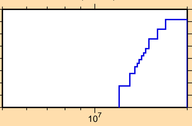
\sigma vs. E for ^{92}\text{Nb}(n,\text{He3})
