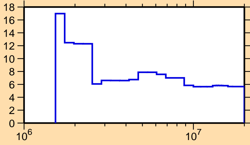
\Delta\sigma/\sigma vs. E for ^{92}\text{Nb}(n,n\text{onel.})
