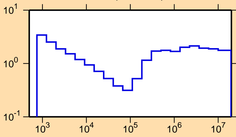
\sigma vs. E for ^{92}\text{Nb}(n,\text{nonel.})
