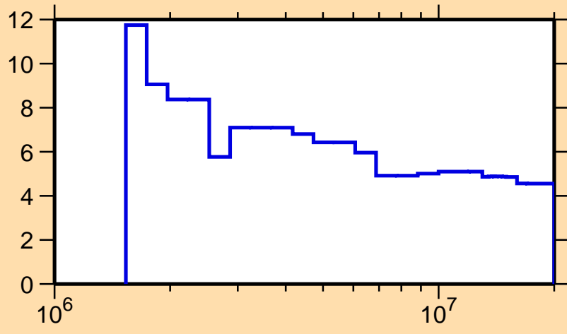
\Delta\sigma/\sigma vs. E for ^{93}\text{Nb}(n,n\text{onel.})
