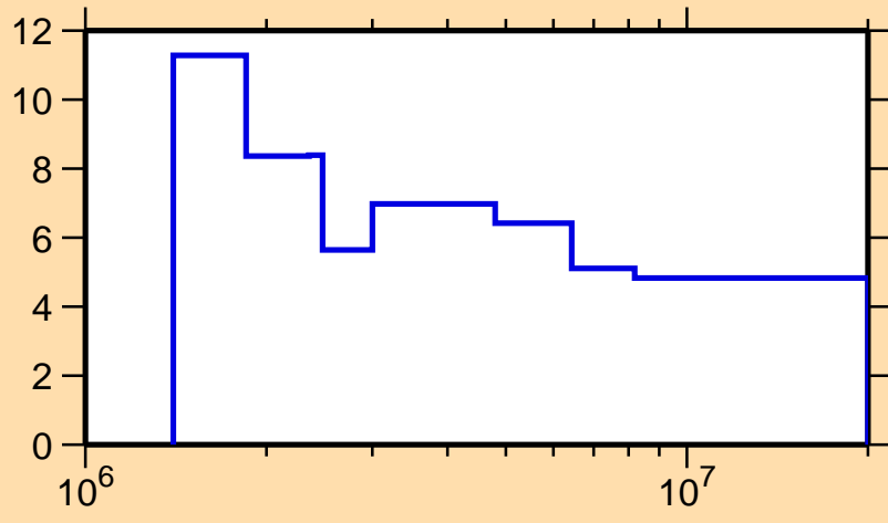
\Delta\sigma/\sigma vs. E for ^{93}\text{Nb}(n,n\text{nonel.})
