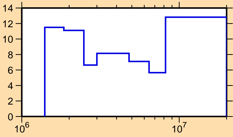
\Delta\sigma/\sigma vs. E for ^{93}\text{Nb}(n,ncont.)
