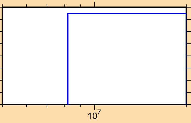
\sigma vs. E for ^{93}\text{Nb}(n,\text{nd})
