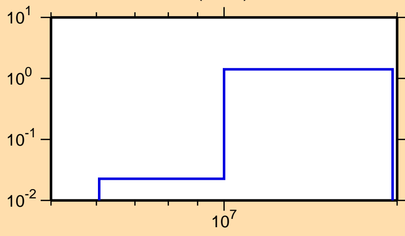
\sigma vs. E for ^{93}\text{Nb}(n,2n)
