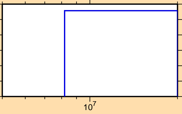
\sigma vs. E for ^{93}\text{Nb}(n,nt)
