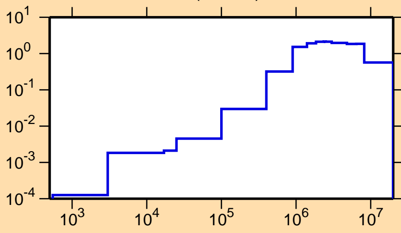
\sigma vs. E for ^{93}\text{Nb}(n,\text{inel.})
