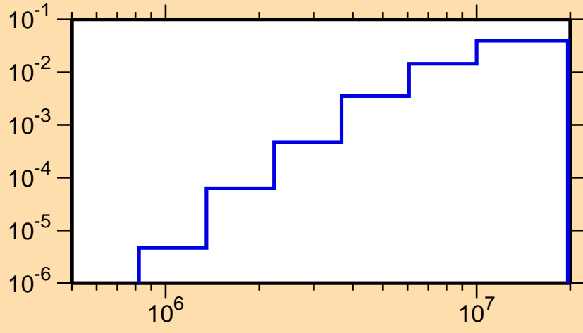
\sigma vs. E for ^{94}\text{Nb}(n,p)
