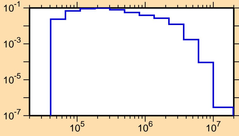
\sigma vs. E for ^{94}\text{Nb}(n,n_1)
