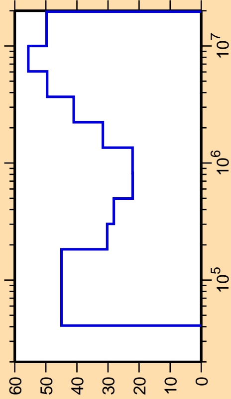
\Delta\sigma/\sigma vs. E for ^{94}\text{Nb}(n,n_2)
