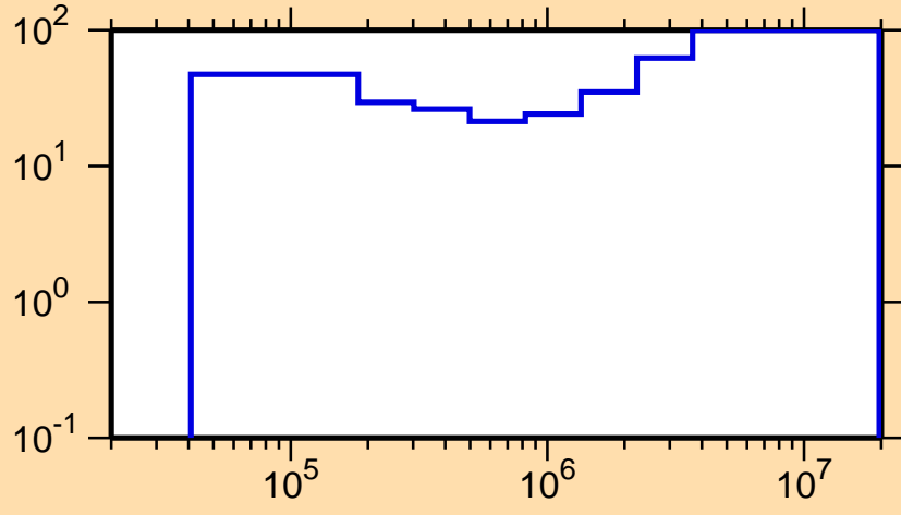
\Delta\sigma/\sigma vs. E for ^{94}\text{Nb}(n,n_1)
