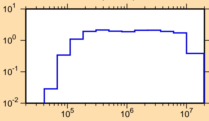
\sigma vs. E for ^{94}\text{Nb}(n,\text{inel.})
