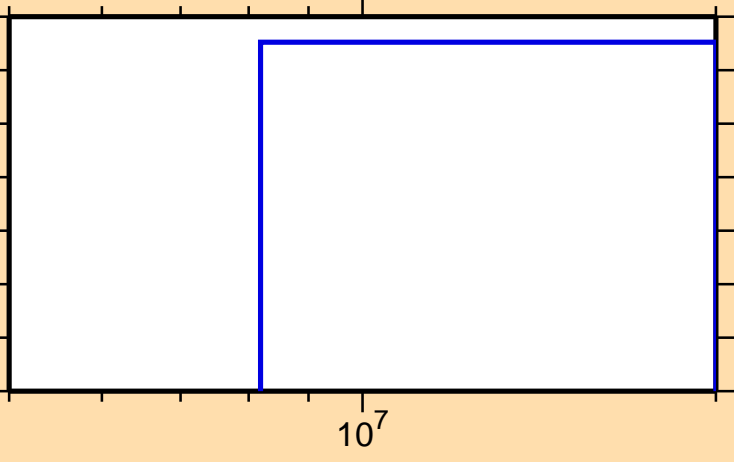
\sigma vs. E for ^{94}\text{Nb}(n,2np)
