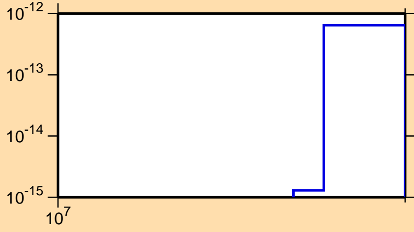
\sigma vs. E for ^{95}\text{Nb} (mt 45)
