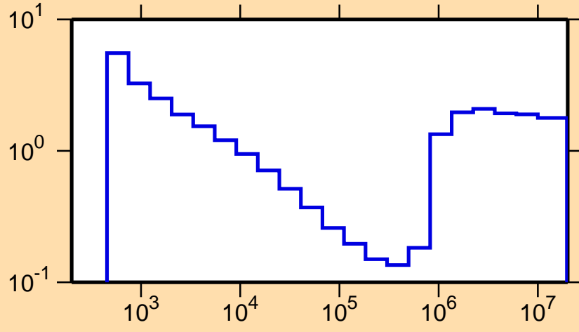
\sigma vs. E for ^{95}\text{Nb}(n,\text{nonel.})
