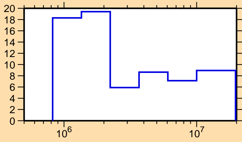
\Delta\sigma/\sigma vs. E for ^{95}\text{Nb}(n,el.)
