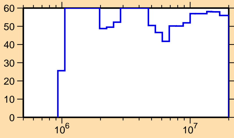
\Delta\sigma/\sigma vs. E for ^{95}\text{Nb}(n,p)
