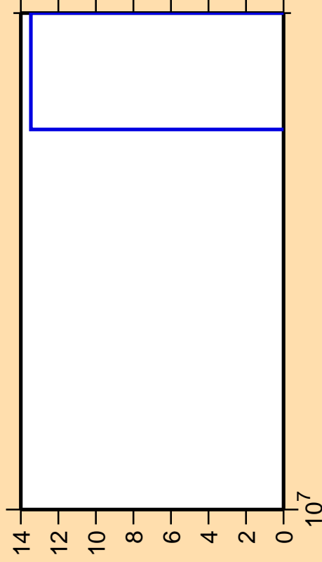
\Delta\sigma/\sigma vs. E for ^{95}\text{Nb} (mt 45)
