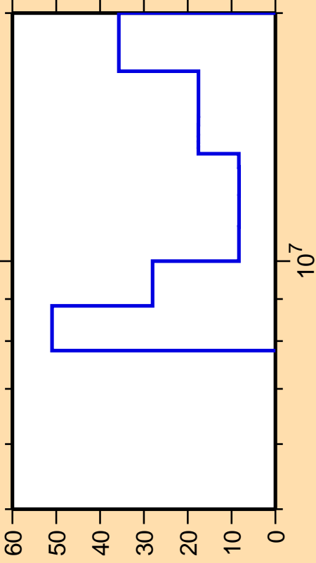
\Delta\sigma/\sigma vs. E for ^{95}\text{Nb}(n,2n)
