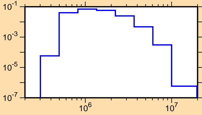
\sigma vs. E for ^{95}\text{Nb}(n,n_2)
