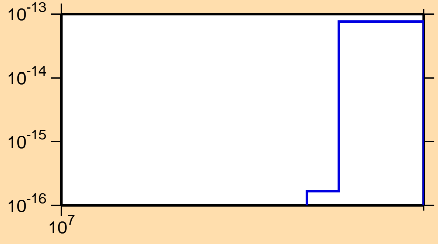
\sigma vs. E for ^{96}\text{Nb}(\text{mt117})
