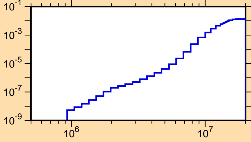
\sigma vs. E for ^{96}\text{Nb}(n,\alpha)
