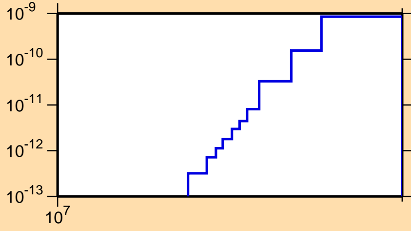
\sigma vs. E for ^{96}\text{Nb}(n,p\alpha)
