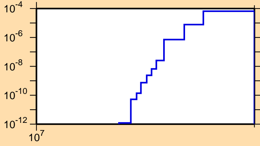
\sigma vs. E for ^{96}\text{Nb}(n,\text{nd})
