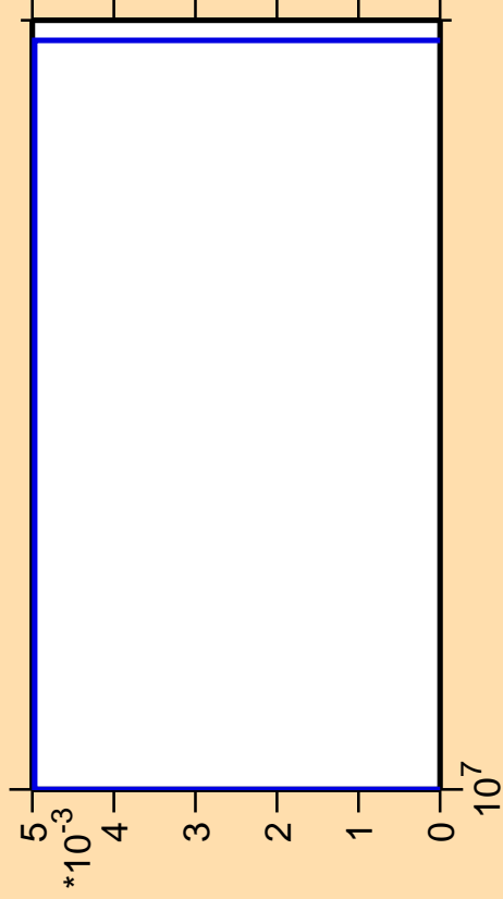
\Delta\sigma/\sigma vs. E for ^{96}\text{Nb}(\text{mt117})
