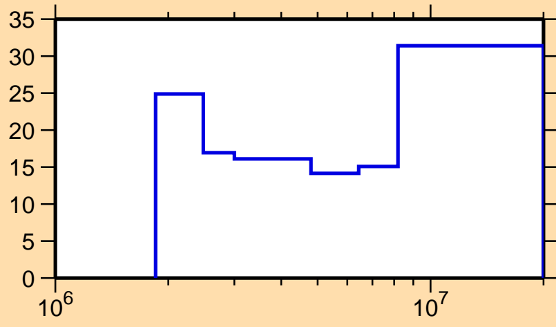
\Delta\sigma/\sigma vs. E for ^{96}\text{Nb}(n,ncont.)
