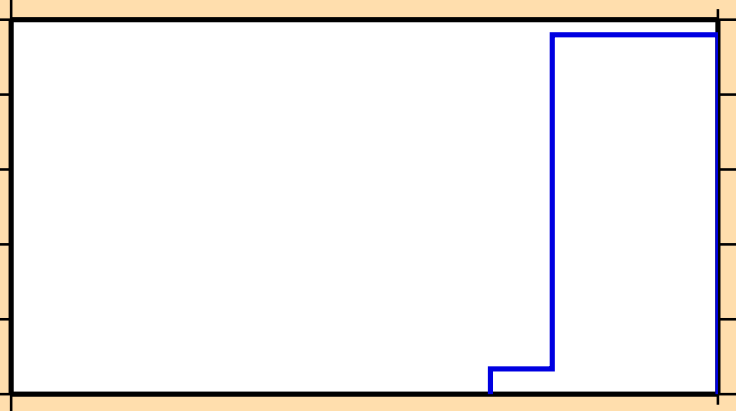
\sigma vs. E for ^{97}\text{Nb}(n,2np)
