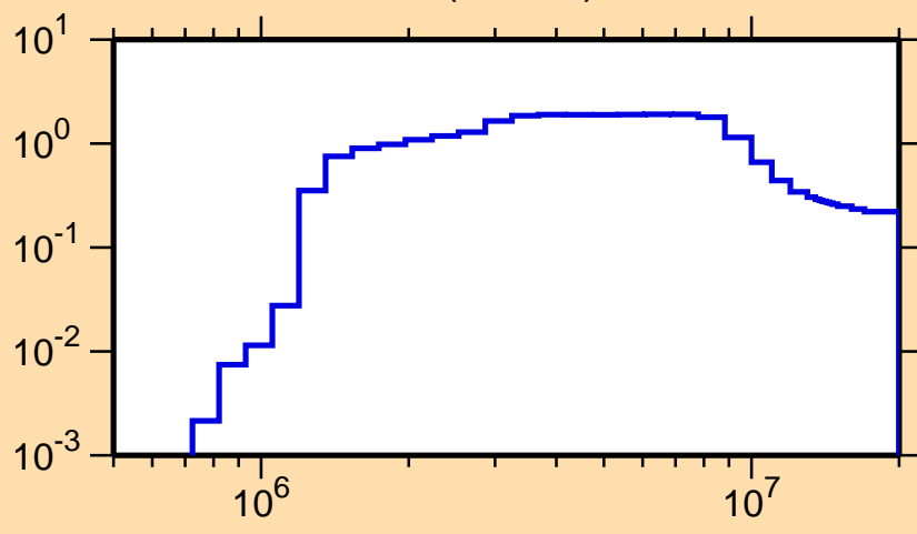
\sigma vs. E for ^{97}\text{Nb}(n,\text{inel.})
