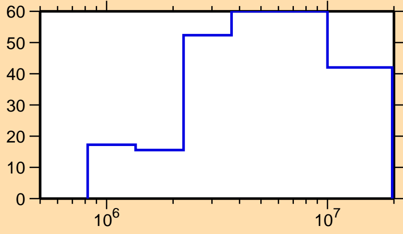
\Delta\sigma/\sigma vs. E for ^{97}\text{Nb}(n,n_1)
