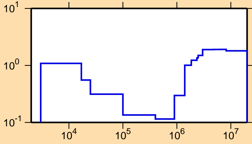
\sigma vs. E for ^{97}\text{Nb}(n,\text{nonel.})
