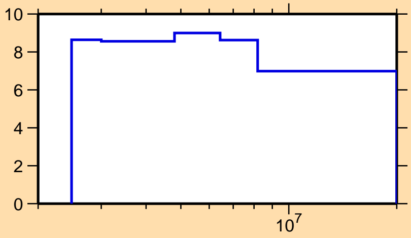
\Delta\sigma/\sigma vs. E for ^{97}\text{Nb}(n,n\text{nonel.})
