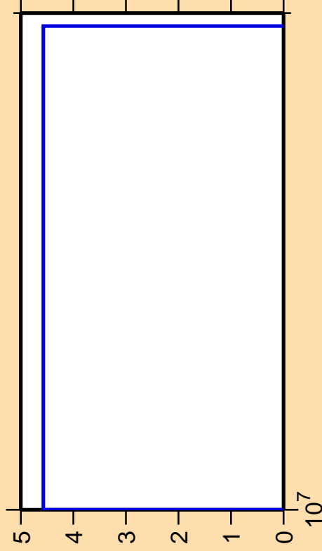
\Delta\sigma/\sigma vs. E for ^{97}\text{Nb}(n,p\alpha)
