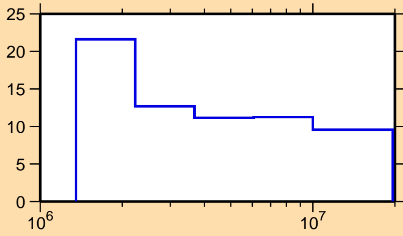
\Delta\sigma/\sigma vs. E for ^{97}\text{Nb}(n,n\text{nonel.})
