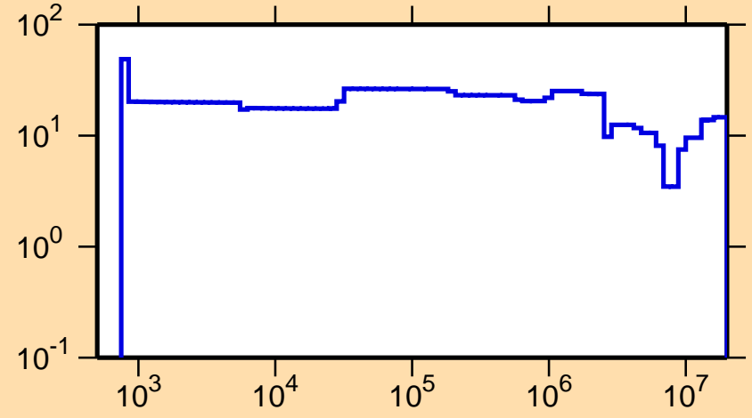
\Delta\sigma/\sigma vs. E for ^{98}\text{Nb}(n,\text{el.})
