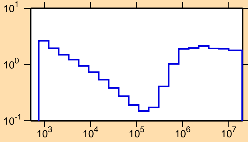
\sigma vs. E for ^{98}\text{Nb}(n,\text{nonel.})
