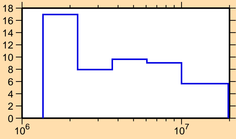
\Delta\sigma/\sigma vs. E for ^{98}\text{Nb}(n,n\text{nonel.})
