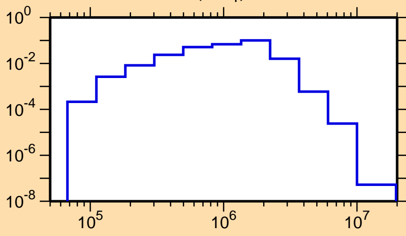
\sigma vs. E for ^{98}\text{Nb}(n,n_1)
