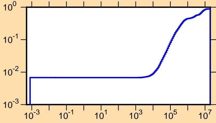
\mu vs. E for ^{99}\text{Nb}(\text{mt251})
