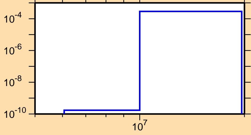
\sigma vs. E for ^{99}\text{Nb}(n,t)
