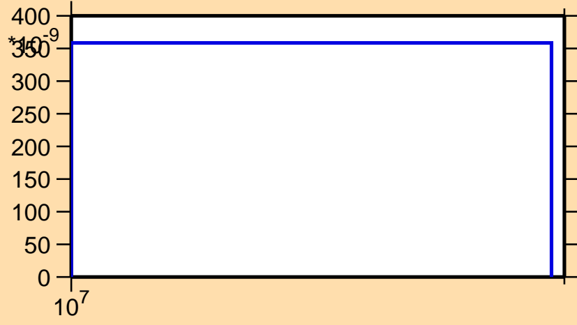
\sigma vs. E for ^{99}\text{Nb}(n,nt)
