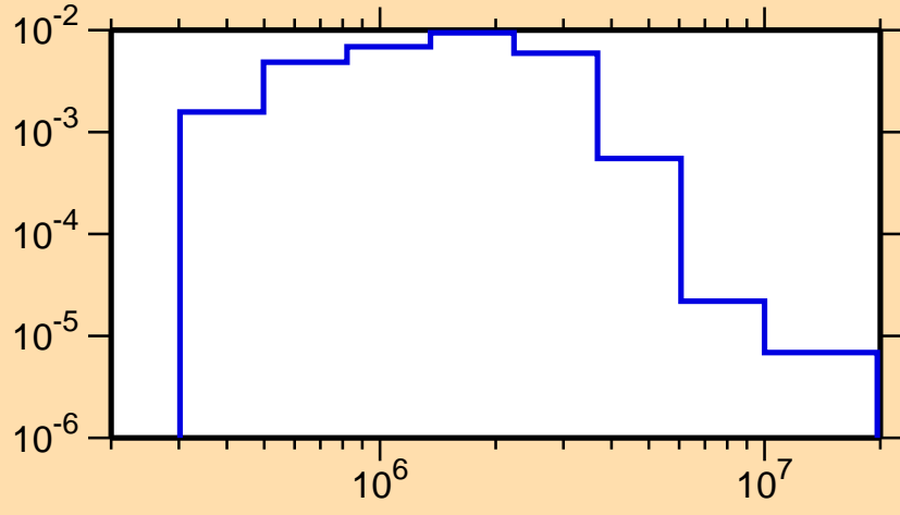
\sigma vs. E for ^{99}\text{Nb}(n,n_1)
