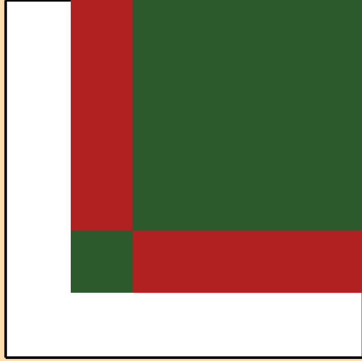
\sigma vs. E for ^{99}\text{Nb}(n,2n)
