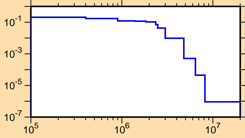
\sigma vs. E for ^{99}\text{Nb}(n,n_3)
