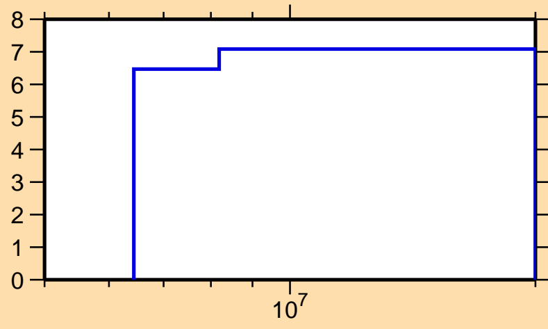
\Delta\sigma/\sigma vs. E for ^{99}\text{Nb}(n,\text{el.})
