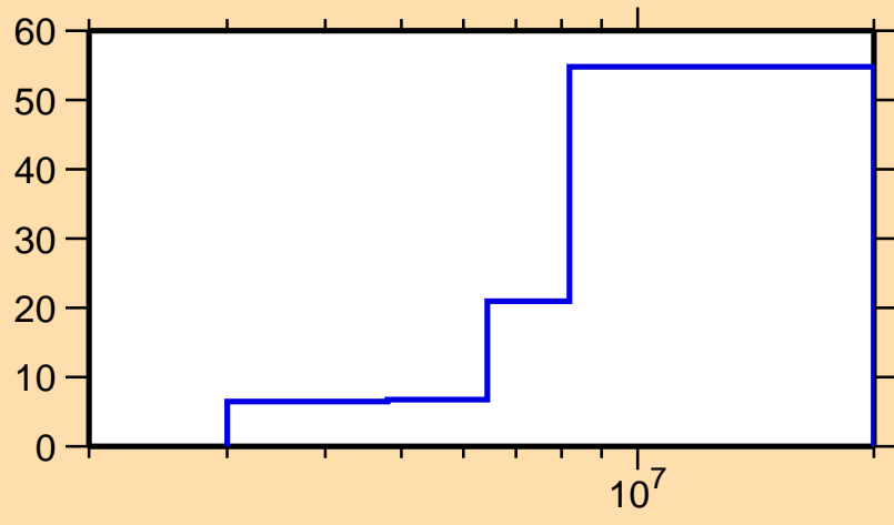
\Delta\sigma/\sigma vs. E for ^{99}\text{Nb}(n,n\text{cont.})
