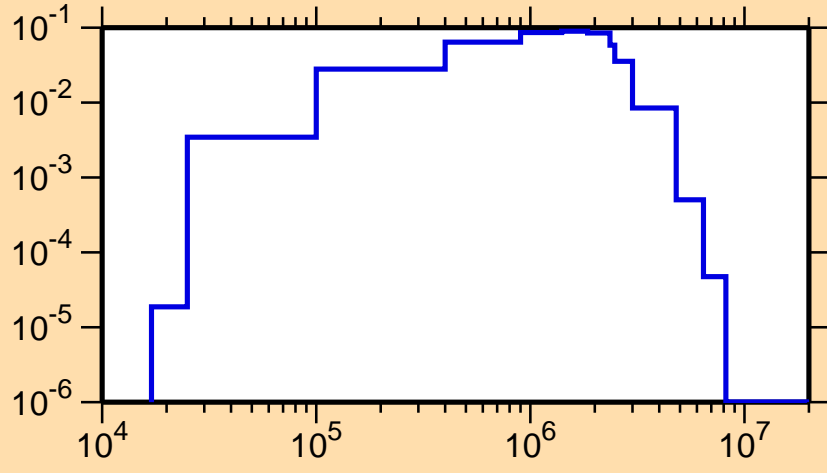
\sigma vs. E for ^{99}\text{Nb}(n,n_2)
