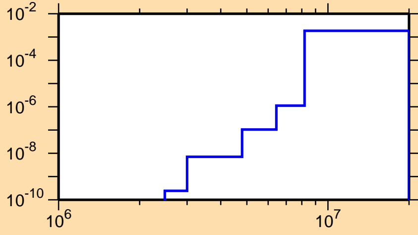
\sigma vs. E for ^{99}\text{Nb}(n,\alpha)
