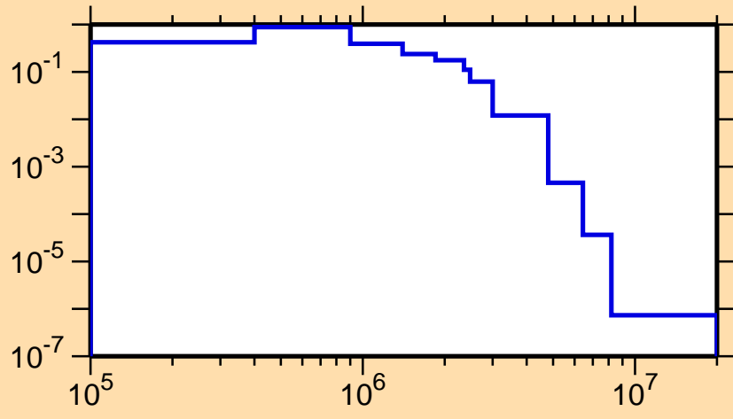
\sigma vs. E for ^{99}\text{Nb}(n,n_4)
