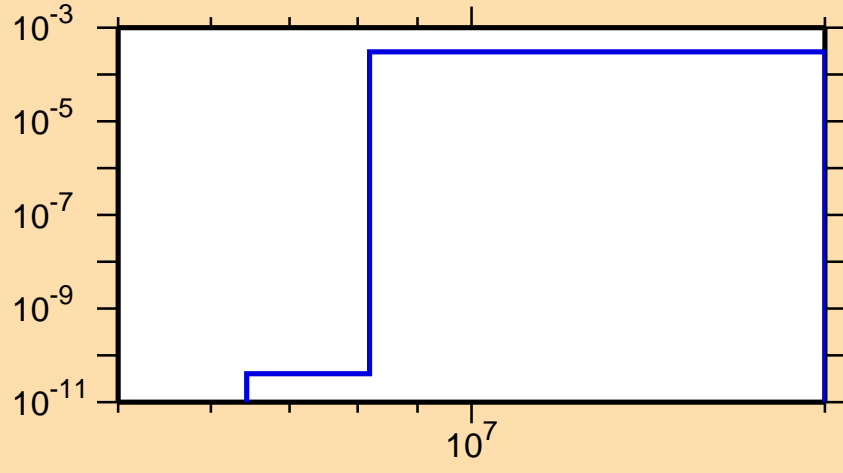
\sigma vs. E for ^{99}\text{Nb}(n,n\alpha)
