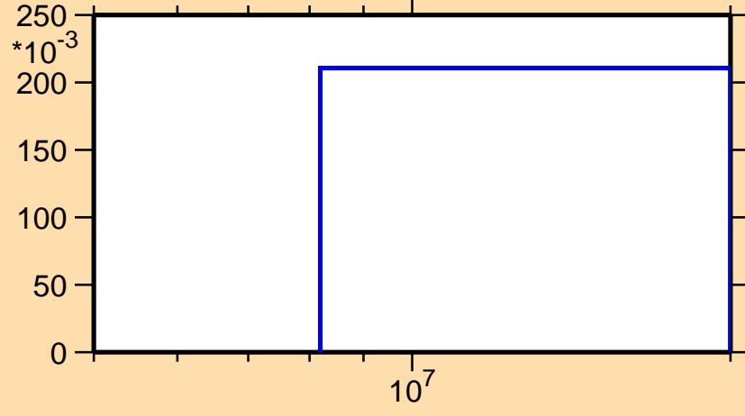
\sigma vs. E for ^{99}\text{Nb}(n,3n)
