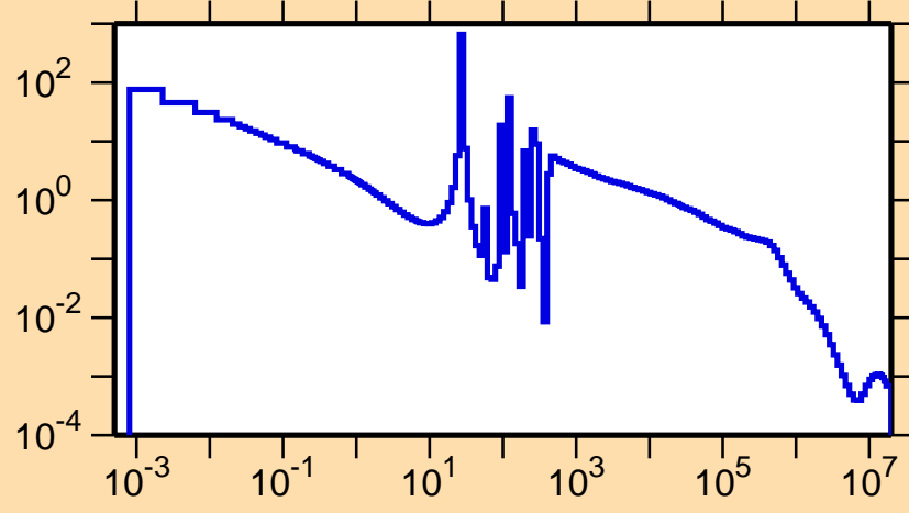
\sigma vs. E for ^{100}\text{Nb}(n,\gamma)
