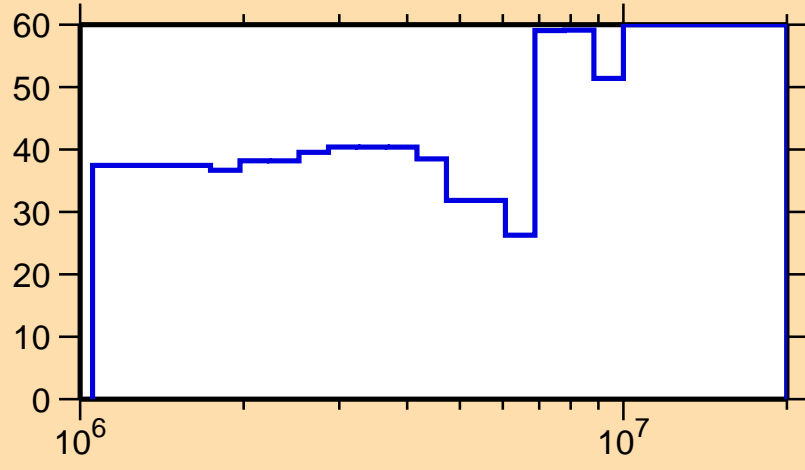
\Delta\sigma/\sigma vs. E for ^{100}\text{Nb}(n,n\text{cont.})
