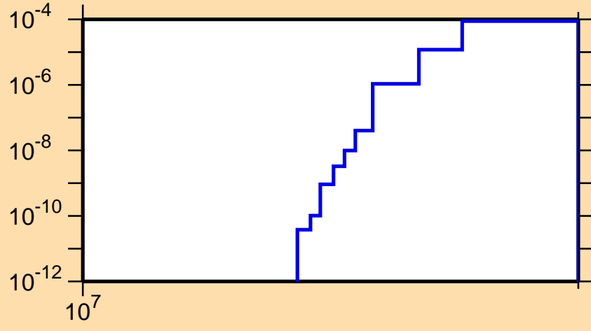
\sigma vs. E for ^{100}\text{Nb}(n,\text{nd})
