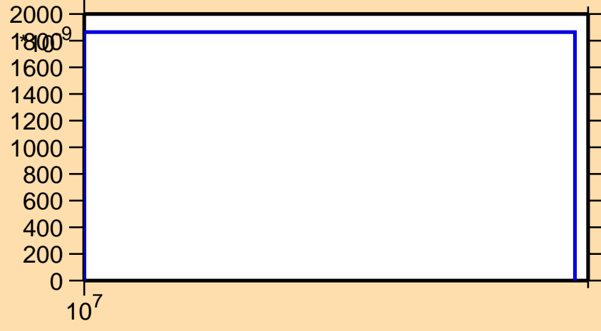
\sigma vs. E for ^{100}\text{Nb}(n,nd)
