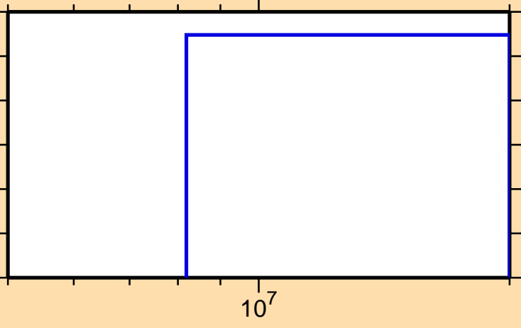
\sigma vs. E for ^{100}\text{Nb}(n,2np)
