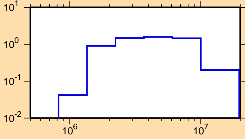
\sigma vs. E for ^{101}\text{Nb}(n,n\text{cont.})
