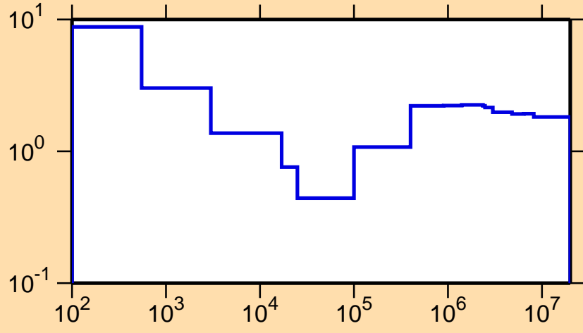
\sigma vs. E for ^{101}\text{Nb}(n,\text{nonel.})
