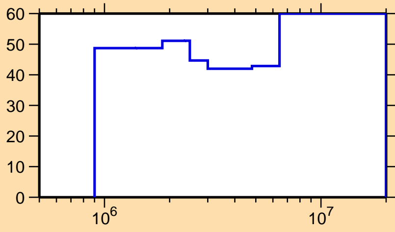
\Delta\sigma/\sigma vs. E for ^{102}\text{Nb}(n,n\text{cont.})
