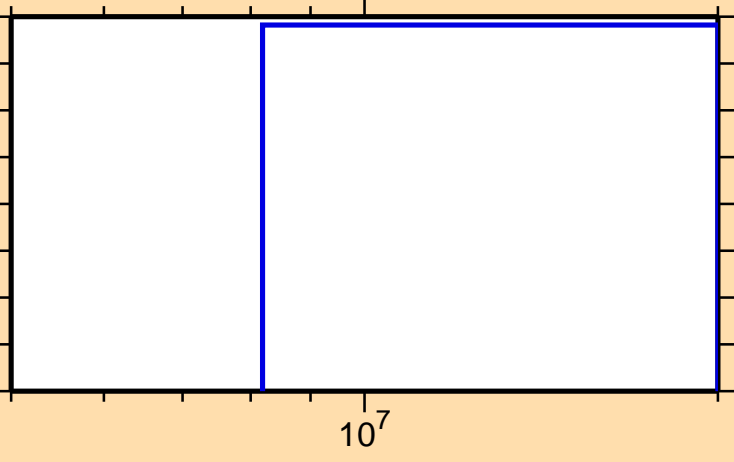
\sigma vs. E for ^{102}\text{Nb}(n,nt)
